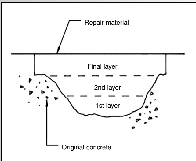
Figure 3: Filling a cavity to ensure that final layer is of uniform thickness
